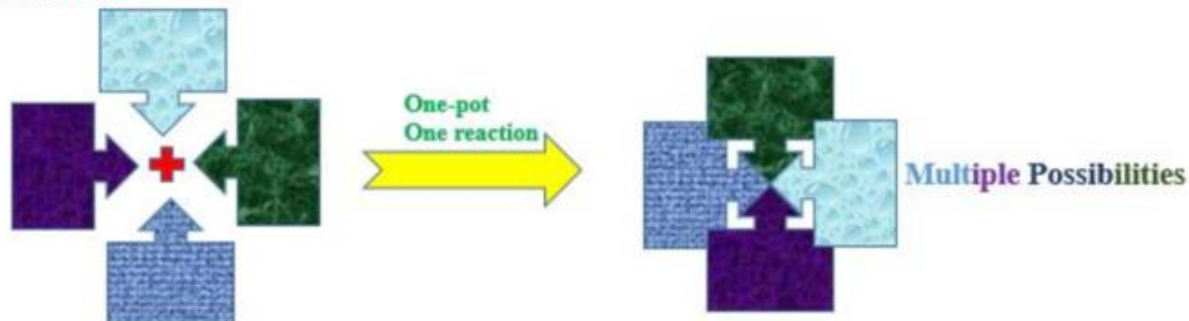
Multicomponent reaction
